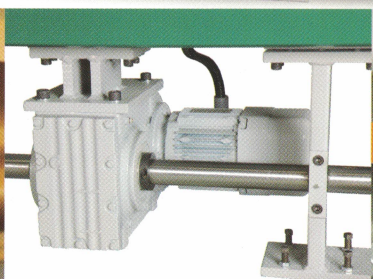
Center motor placement maximizes power while reducing torque loss through the drive shaft.
